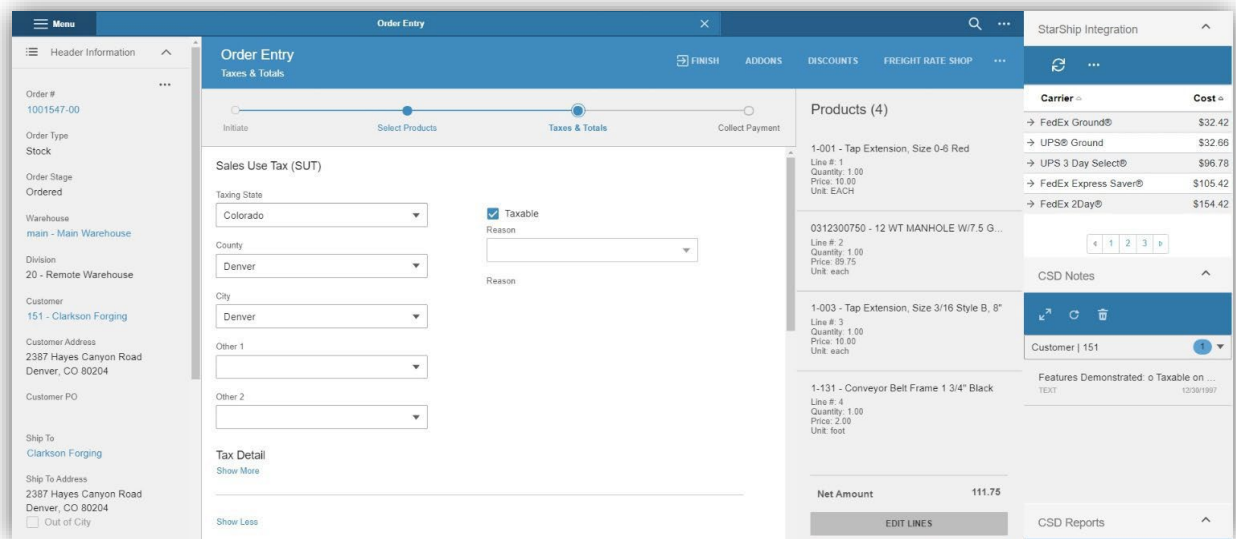
This is a CloudSuite Order Entry screenshot with the optional freight rate shopper plug-in for Starship so the user can shop freight rates while taking the customer's order.
